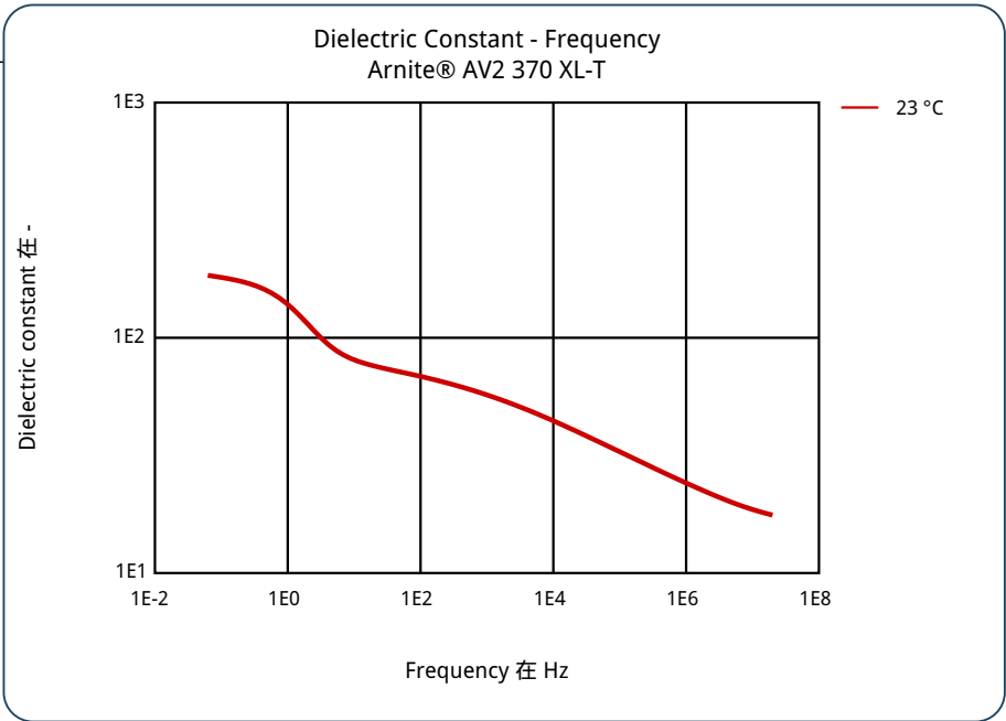
Dielectric Constant - Frequency
